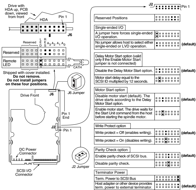
Note. LC drives cannot be configured to provide termination power to the bus. Figure 2. LW/LC option select jumpers
