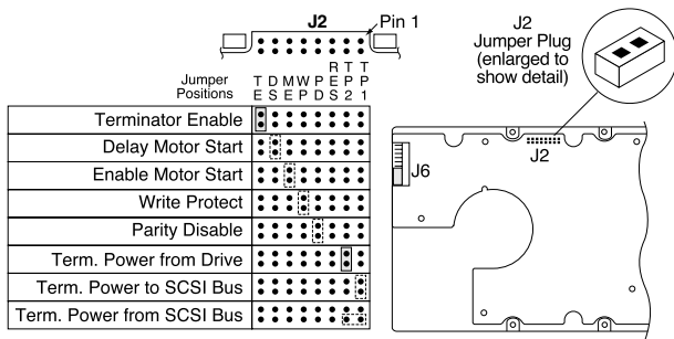
Figure 3. NW option select jumpers
